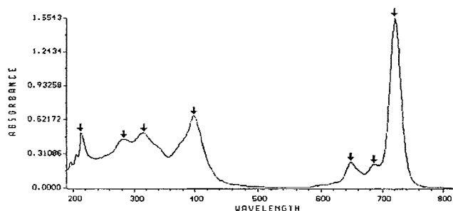
Fig. 2. The UV-vis absorption spectrum of Pc 19.
