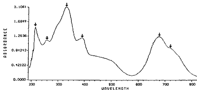
Fig. 1. The UV-vis absorption spectrum of Pc 18.
