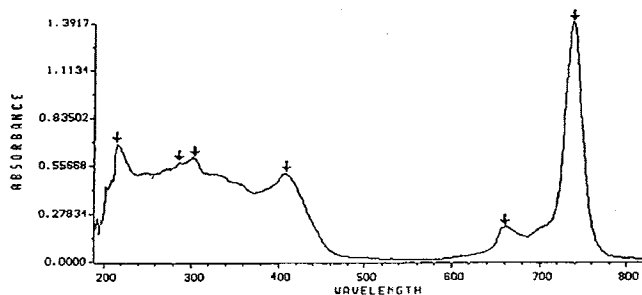
Fig. 4. The UV-vis absorption spectrum of Pc 26.
