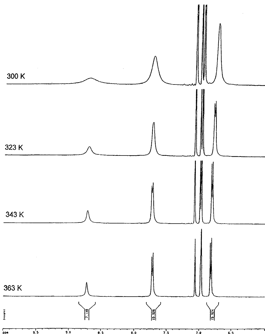
Fig. 3. The temperature dependent ^1\text{H} NMR spectra of Pc 18.
