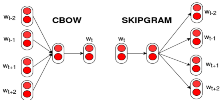
Figure 2.2: CBOW and Skipgram for training Word2vec word embedding, by Aeluo13 [CC BY-SA 4.0 ( https://creativecommons.org/licenses/by-sa/4.0 )], from Wikimedia Commons
