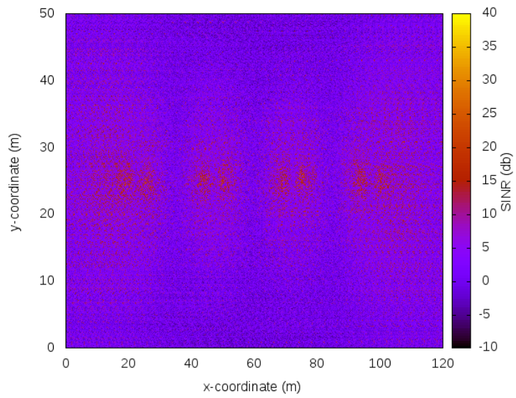
Figure 4.29: Wi-Fi/LAA radio environment map.
