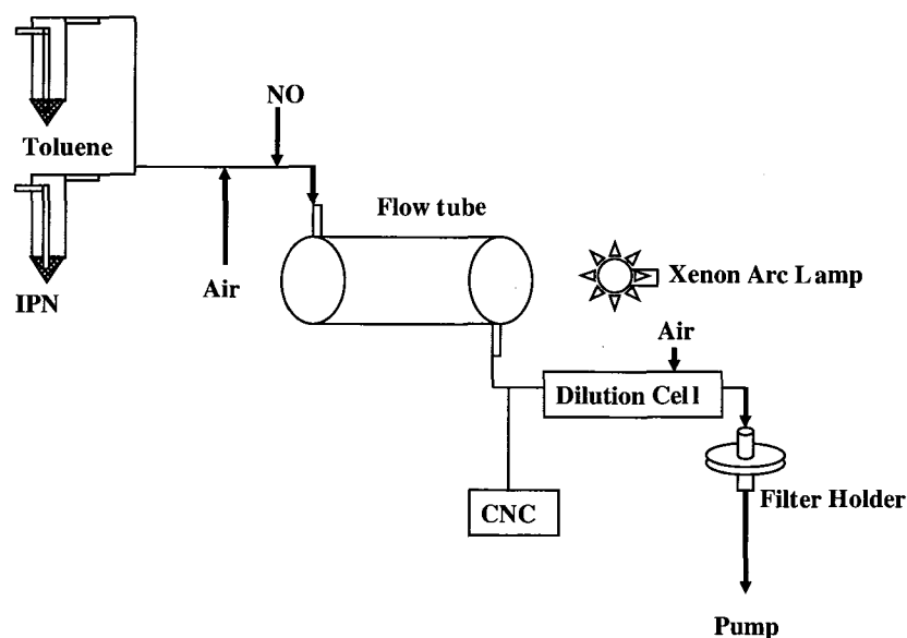
Fig. 1. Schematic diagram for the flow reactor experiment; see text for detailed explanations.
