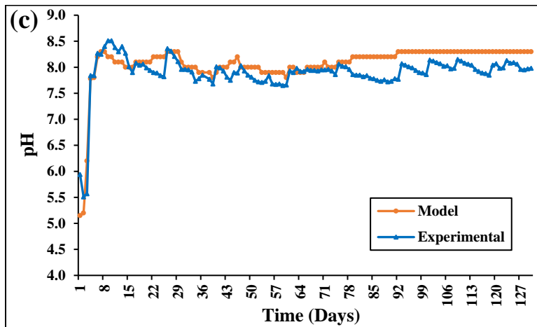
Figure 4-4: Comparison between daily effluent measured and dynamic model data for: (a) Nitrite concentrations; (b) nitrate concentrations; (c) pH
