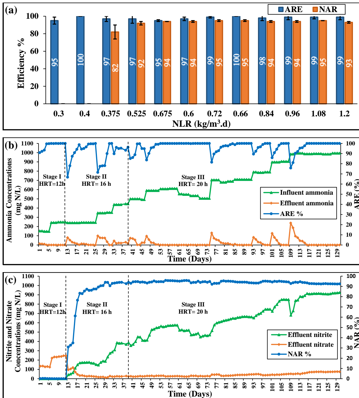
Figure 3-2: SBR Nitrogen removal performance during the three stages of operation: (a) Ammonia Removal Efficiency (ARE) and Nitrite Accumulation rate (NAR) during different NLR; (b) Influent and Effluent NH 3 -N concentrations and ammonia removal efficiency; (c) NO 2 -N and NO 3 -N concentrations in the effluent and NAR (%)
