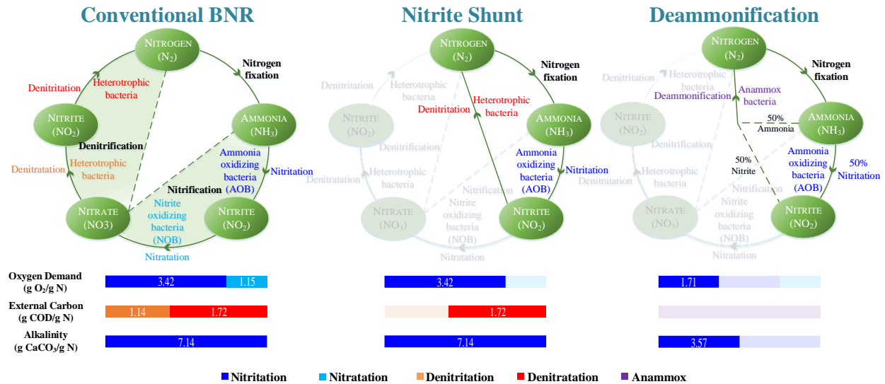
Figure 1-1: Comparison between conventional and shortcut nitrogen removal over the nitrogen cycle
