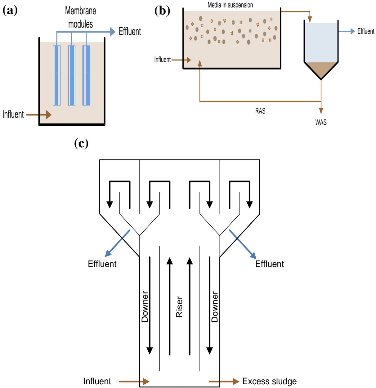
Figure 2-5: Biofilm reactor configurations. (a) MBR; (b) MBBR; (c) BAS
