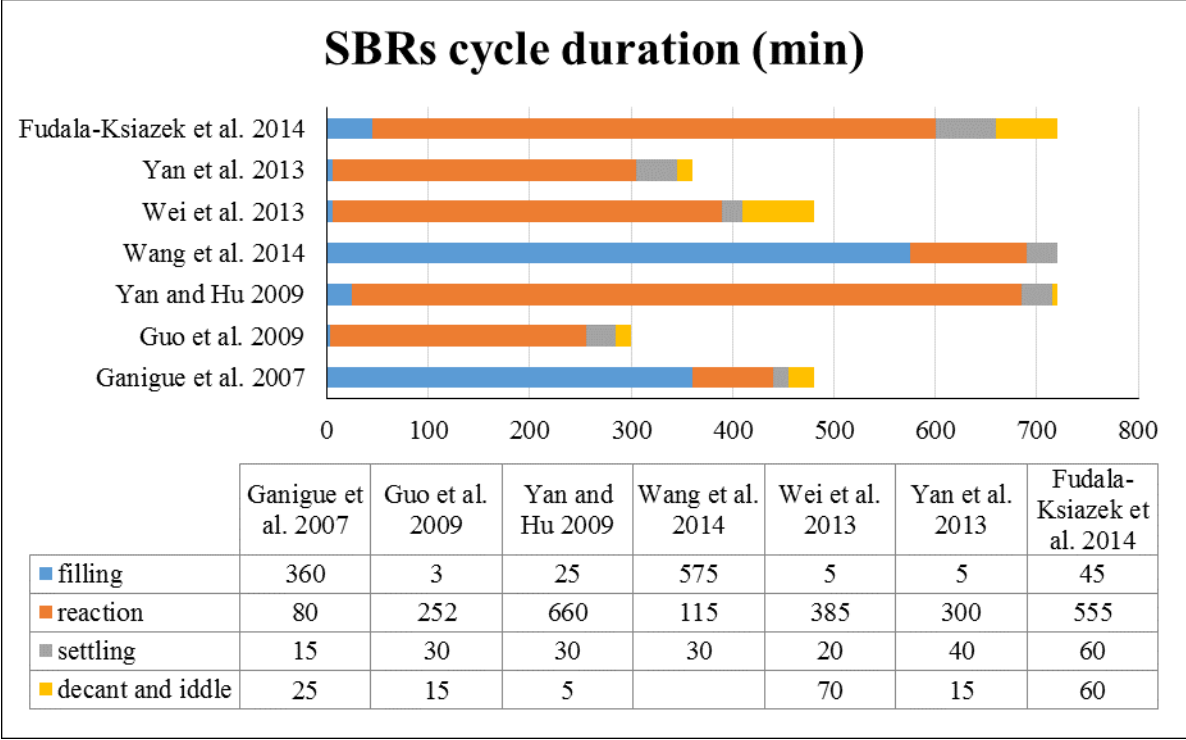
Figure 2-4: SBR cycle duration for different partial nitrification studies
