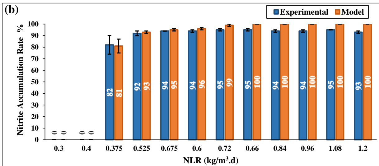
Figure 4-3: Comparison between experimental and model data during different Nitrogen loading levels (NLR) in terms of: (a) Ammonia removal efficiency (ARE), (b) Nitrite accumulation rate (NAR)
