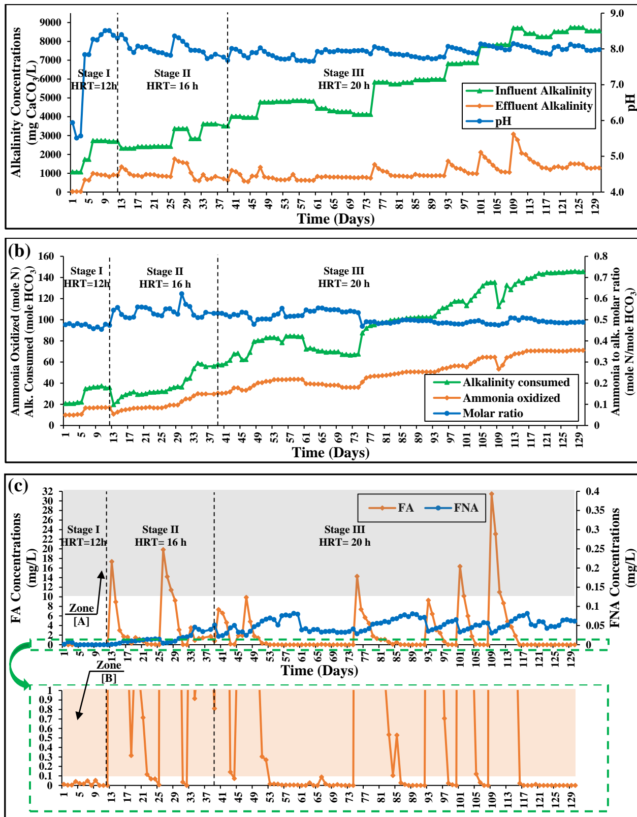
Figure 3-3: Typical profile for: (a) influent alkalinity concentrations, effluent alkalinity concentrations and pH, (b) oxidized ammonia to alkalinity consumed molar ratio, and (c) free ammonia (FA) and free nitrous acid (FNA) concentrations where Zone [A]: FA inhibition to AOB and Zone [B]: FA inhibition to NOB
