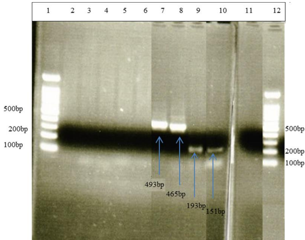
Figure 3-4: PCR products using genomic DNA of sample 1 and 2 with the five sets of primers.
