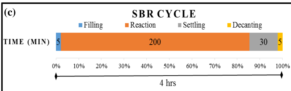
Figure 3-1: (a) Schematic Diagram of the SBR used in this experiment; (b) BioFlo ® 115 Benchtop Fermenter & Bioreactor during operation; (c) SBR's cycle for Partial Nitrification process
