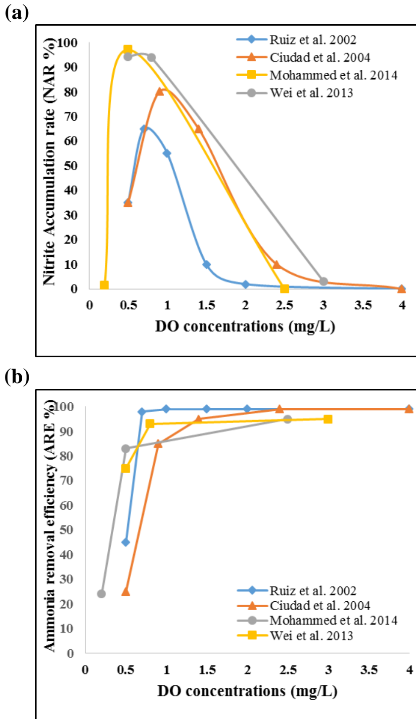
Figure 2-3: Performance of Partial nitrification suspended systems during different DO concentrations in terms of: (a) Nitrite accumulation rate (NAR); (b) Ammonia removal efficiency (ARE)
