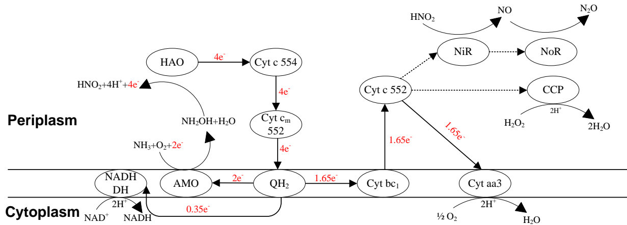
Figure 2-2: Electron transport pathways in AOB
