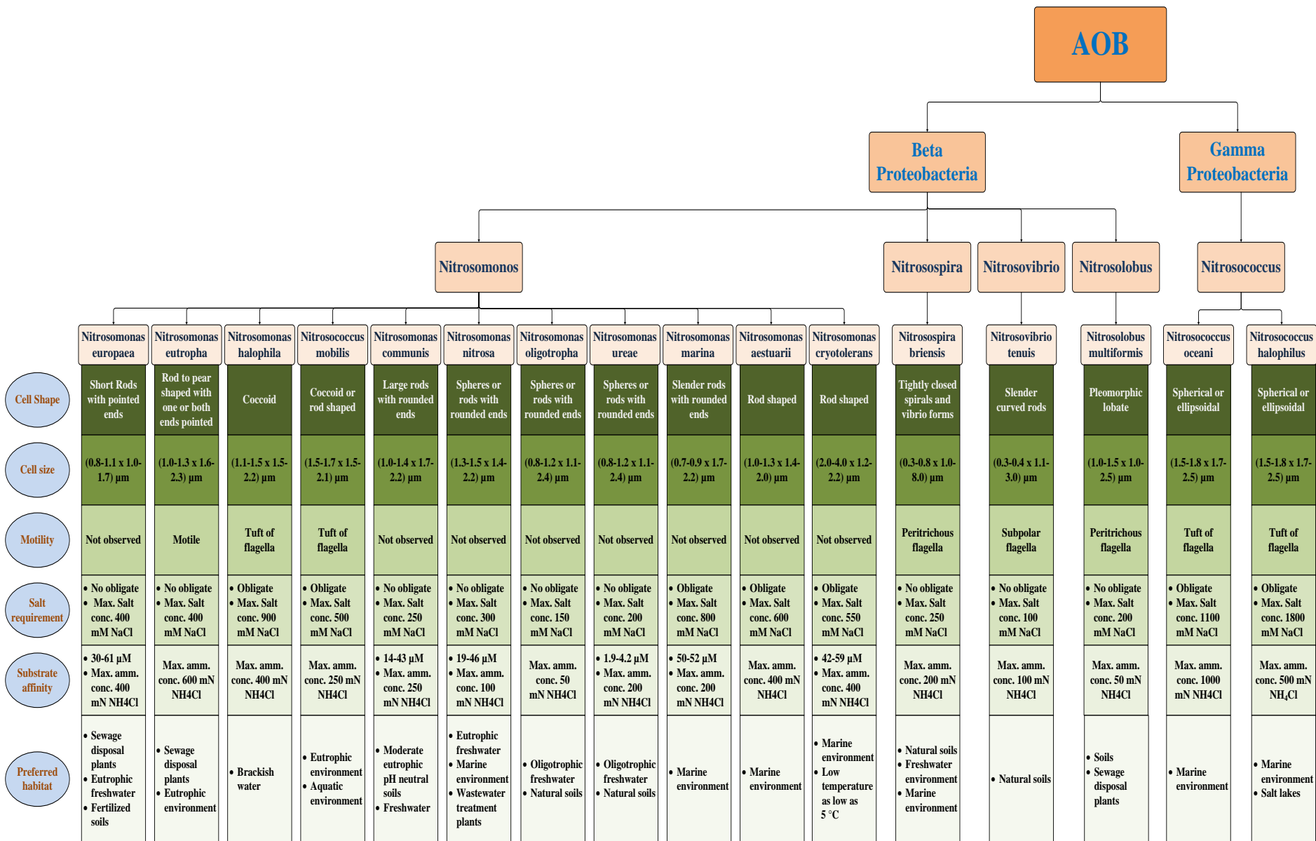
Figure 2-1: Morphological and Eco-physiological Characteristics of reported Ammonia Oxidizing Bacteria's species
