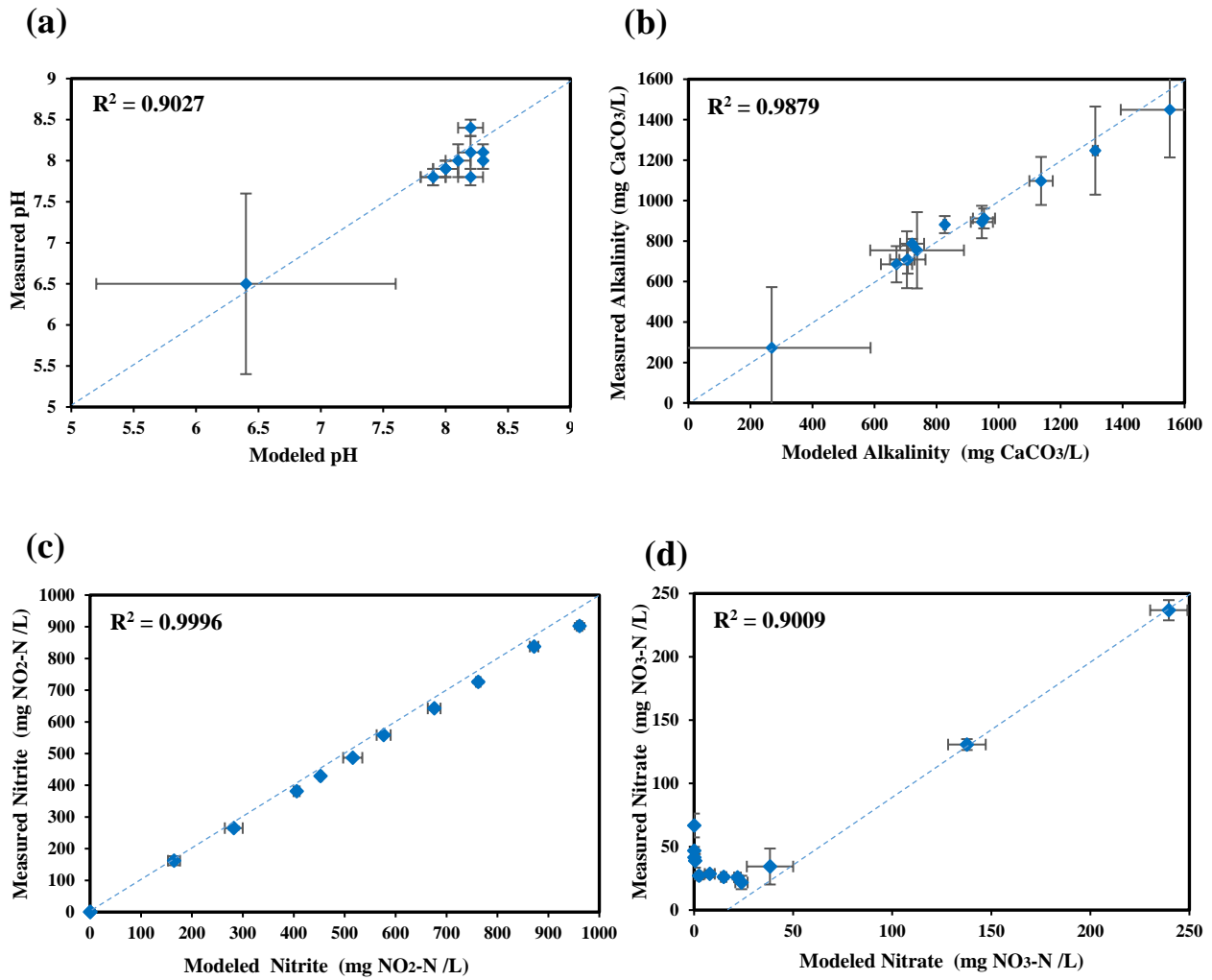
Figure 4-2: Correlation between model and measured effluent parameters for: (a) pH, (b) alkalinity, (c) nitrite, (d) nitrate (Note: vertical and horizontal error bars represent the standard deviations for the measured and model results, respectively)
