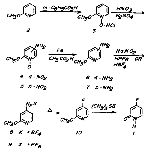
SCHEME I
