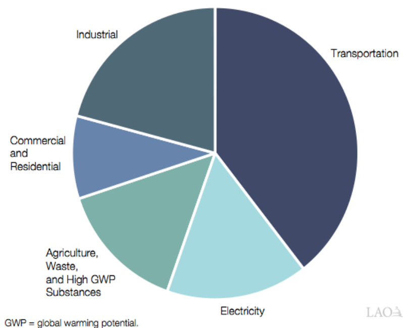
Figure 5. California GHG Emissions since in 2018 by sector (Taylor 2018).
