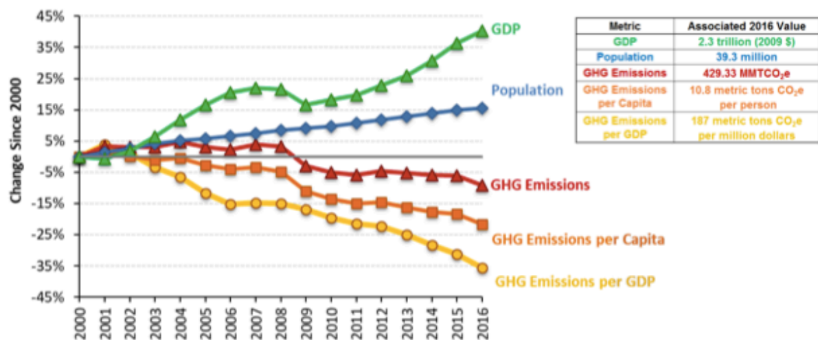
Figure 3. California’s GHG emissions, population, GDP, GHG per capita and carbon intensity of the economy since the year 2000 (CARB 2018).
