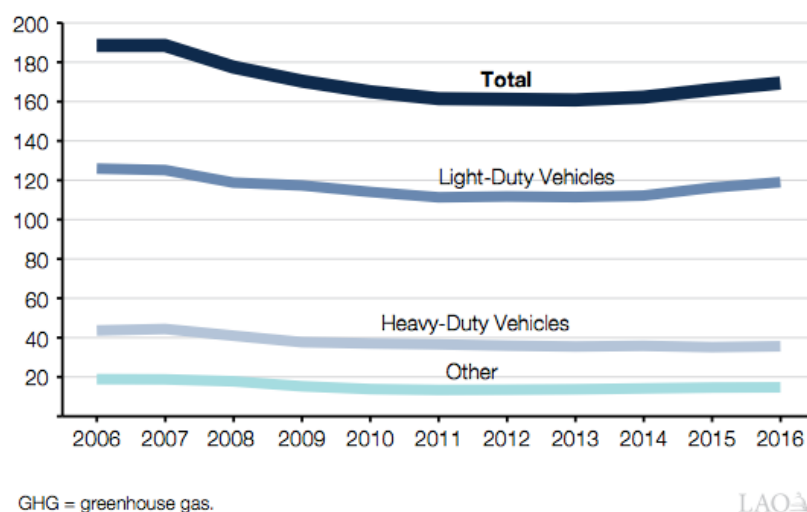
Figure 4. California Transportation Emissions in Million Metric Tons (Taylor 2018).
