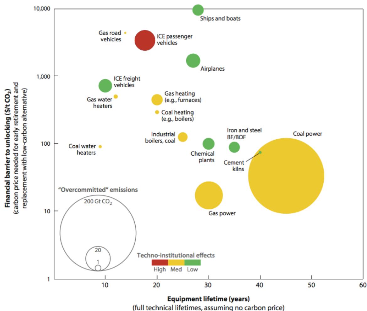
Figure 22. Assessed lock in of various types of CO 2 emitting infrastructure, plotted according to their historical lifetime (x-axis) and the carbon price required to equalize the marginal cost (mainly fuel) and total levelized cost (operating and capital costs) of the existing infrastructure of a low-carbon replacement (y-axis) (Erickson et al. 2015).
