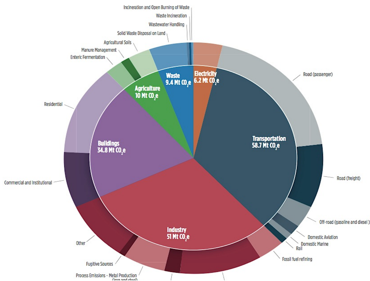
Figure 2. Ontario GHG Emissions in 2014 by sector (Environment and Climate Change Canada 2016; cited in ECO 2016).
