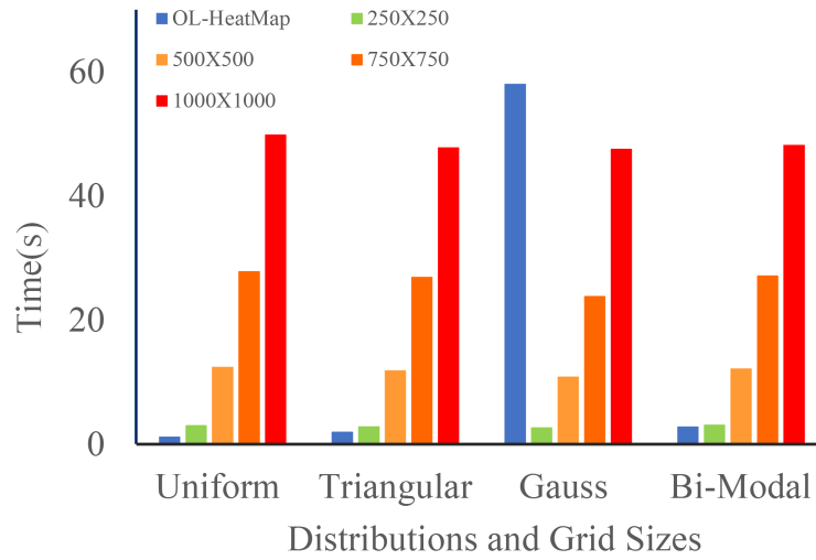
(b) Comparison of time for different data distributions
