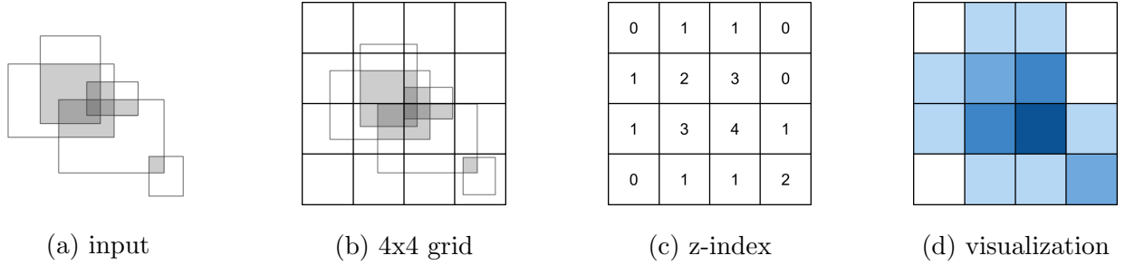
Figure 4.1: Overview of the grid-based method.
