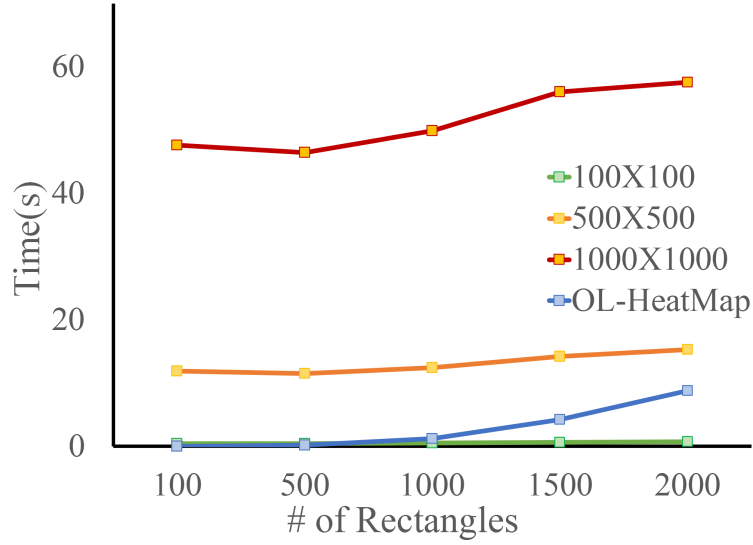
(a) Comparison of time for different data-set sizes
