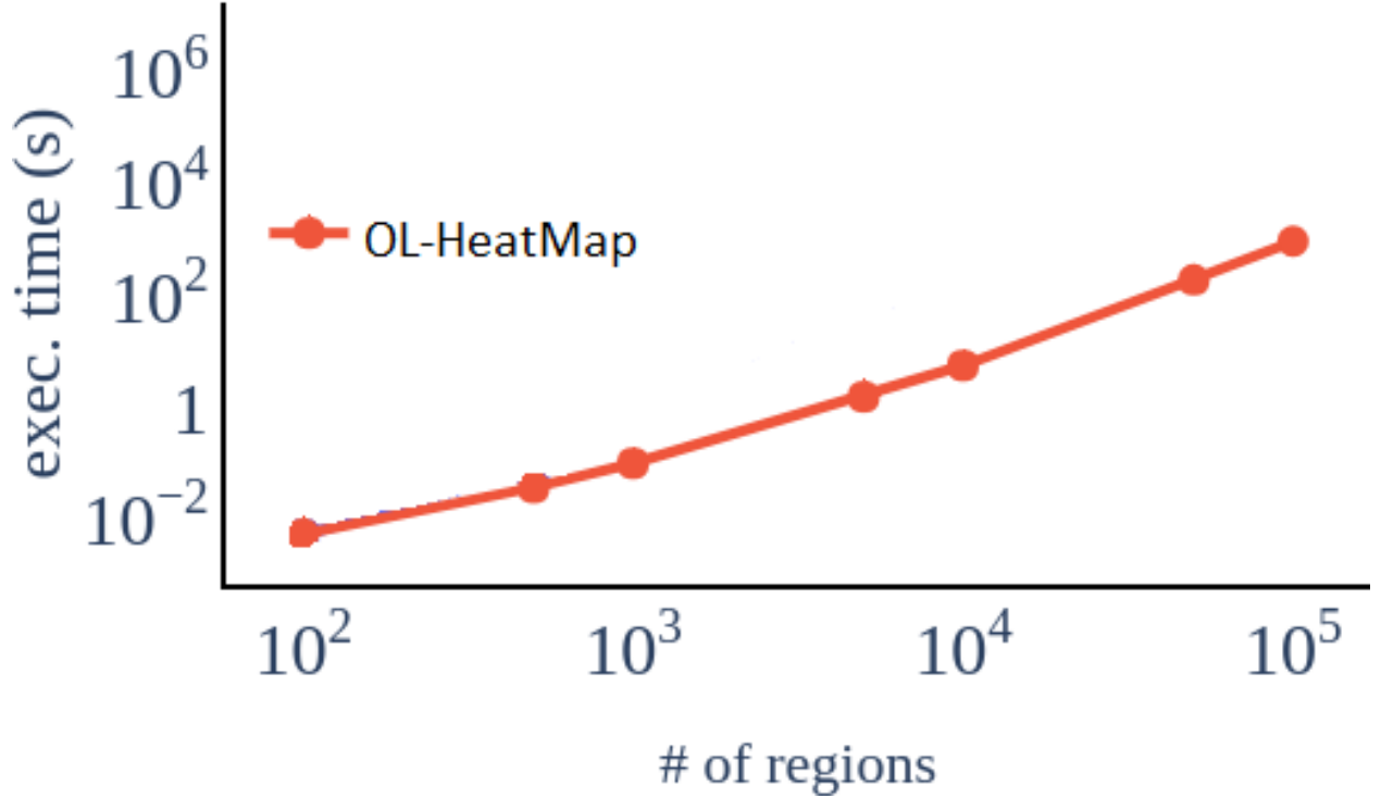
Figure 5.6: Scalability analysis
