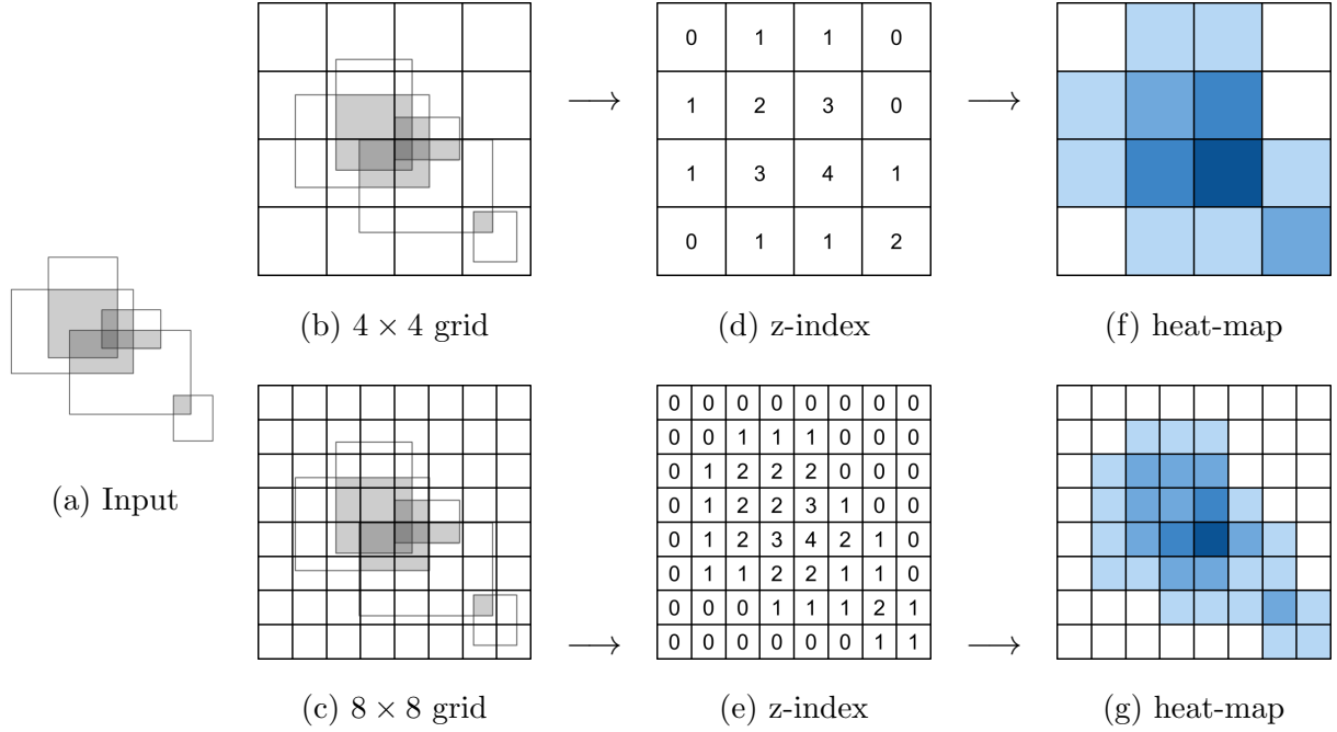
Figure 3.1: Grid construction and z-index calculation for different values of g .
