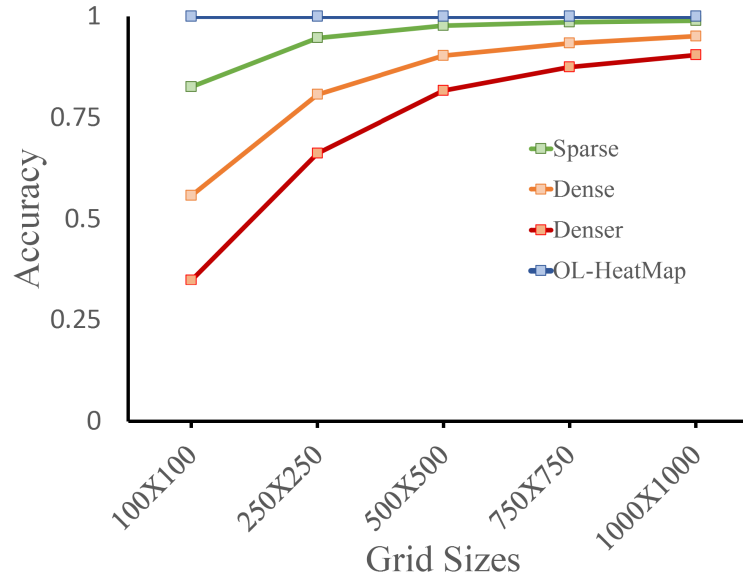
(a) Measurement of accuracy for different grid sizes
