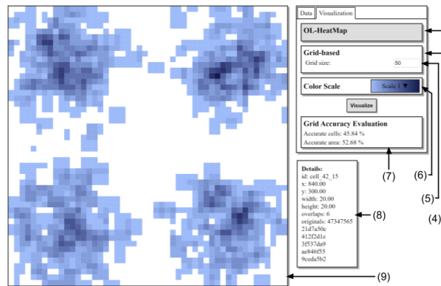
(b) Grid-based visualization
