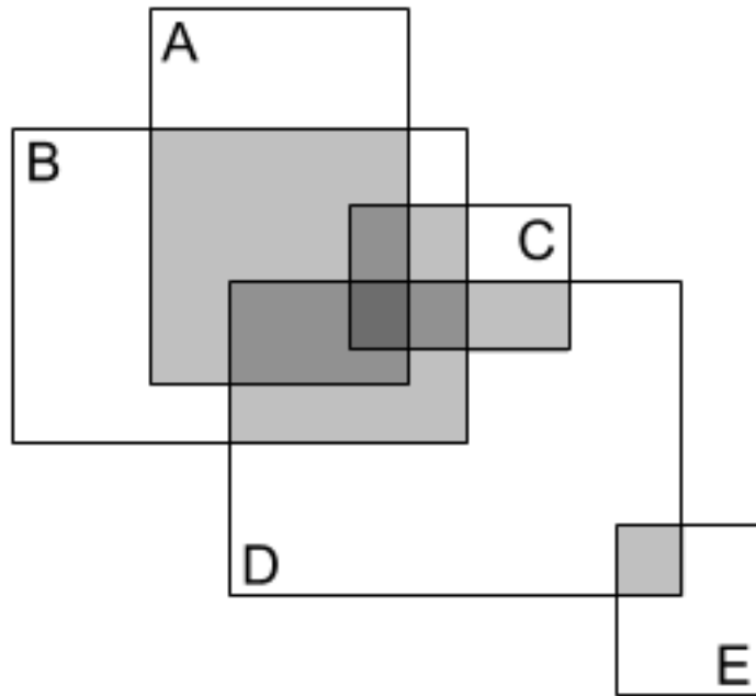
Figure 1.1: Illustrative example of a few overlapping rectangles. We propose effective methods (fast and exact) for a density-based visualization of the multiple overlaps.
