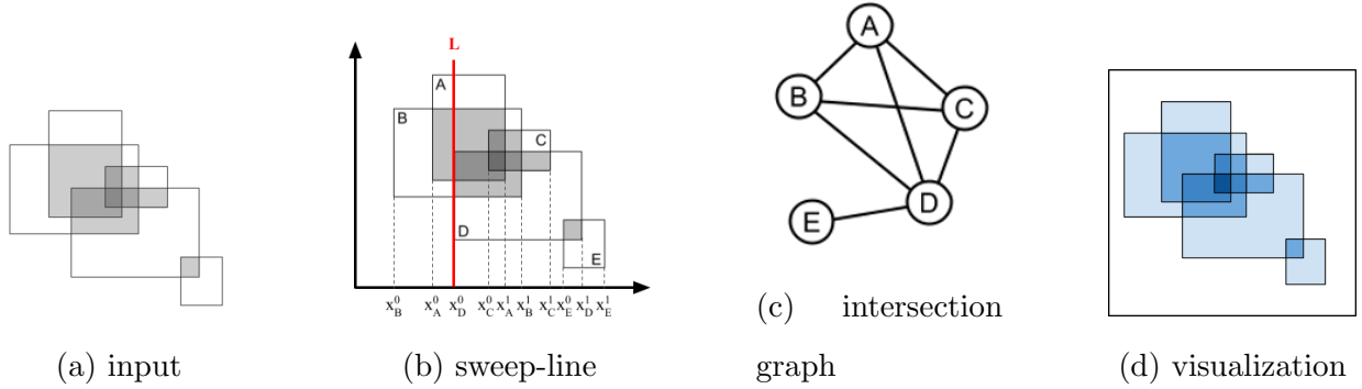
Figure 4.3: Overview of the OL-HEATMAP method.
