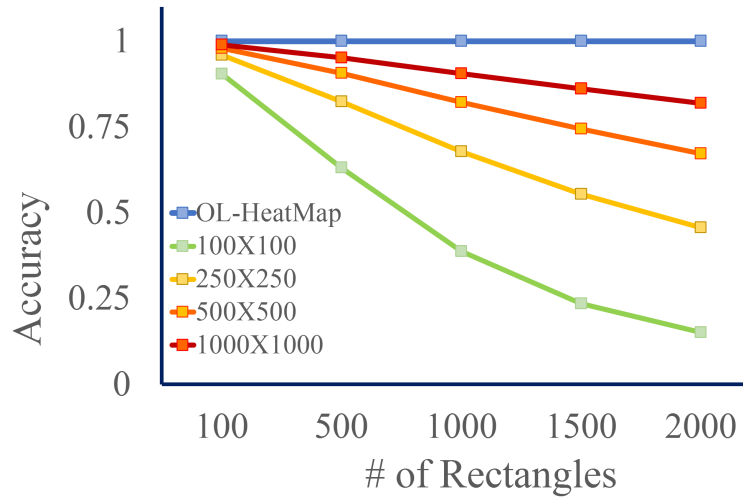
(b) Measurement of accuracy for different data-set sizes
