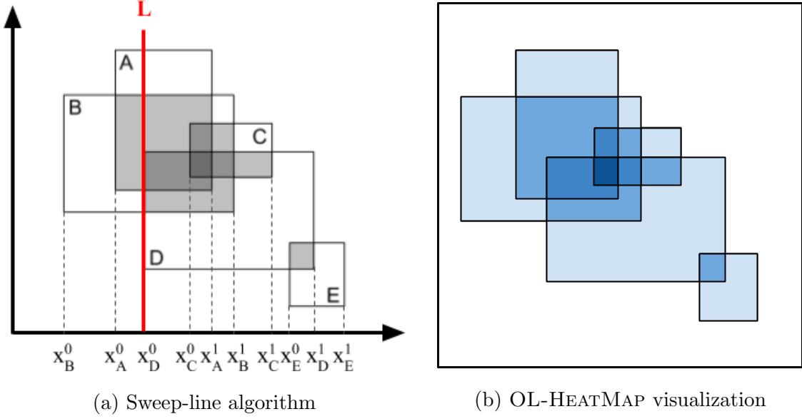
Figure 4.2: Illustrative example of a sweep-line algorithm and resulting OL-HEATMAP visualization.
