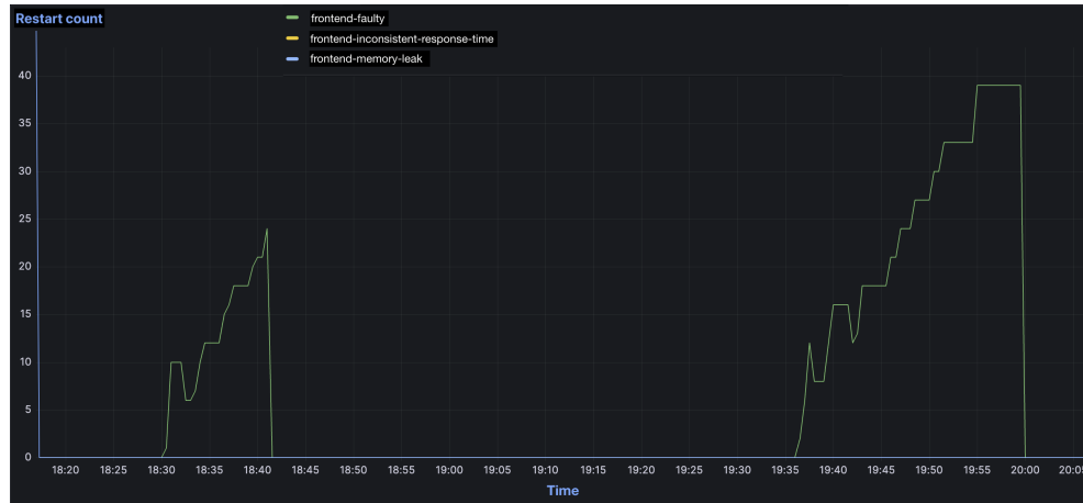
Figure 4.4: Restart count of frontend microservice versions. This chart illustrates the frequency and patterns of system restarts over a specific period.
