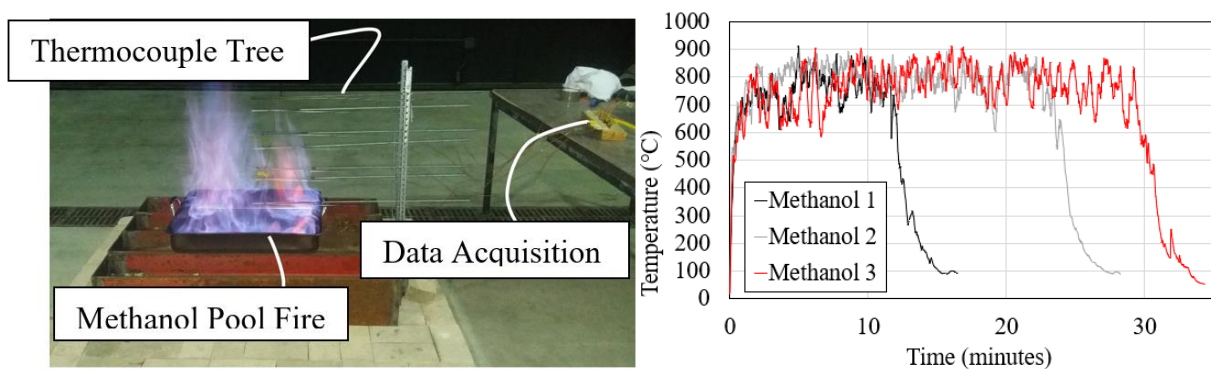
Figure 4.7 Characterization of methanol non-standard fire, where Methanol 1, 2, and 3 represent the trials considered in determining the volume of fuel required ( h = 200 mm).
