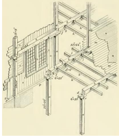
Figure 5.3 Detail of a slow-burning construction building (from A Treatise on Architecture and Building Construction) [74].
