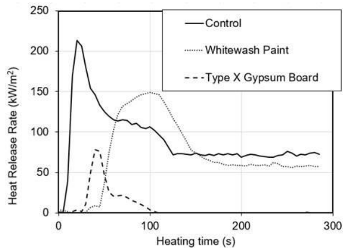
Figure 3.9 Heat release rates over time for the control, whitewash, and gypsum board encapsulations.
