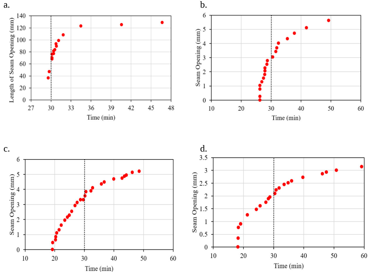
Figure 4.23 Seam opening in the heating and cooling phases (left and right of the dashed lines) for a. Column 2, b. Column 3, c. Column 4, and; d. Column 5.
