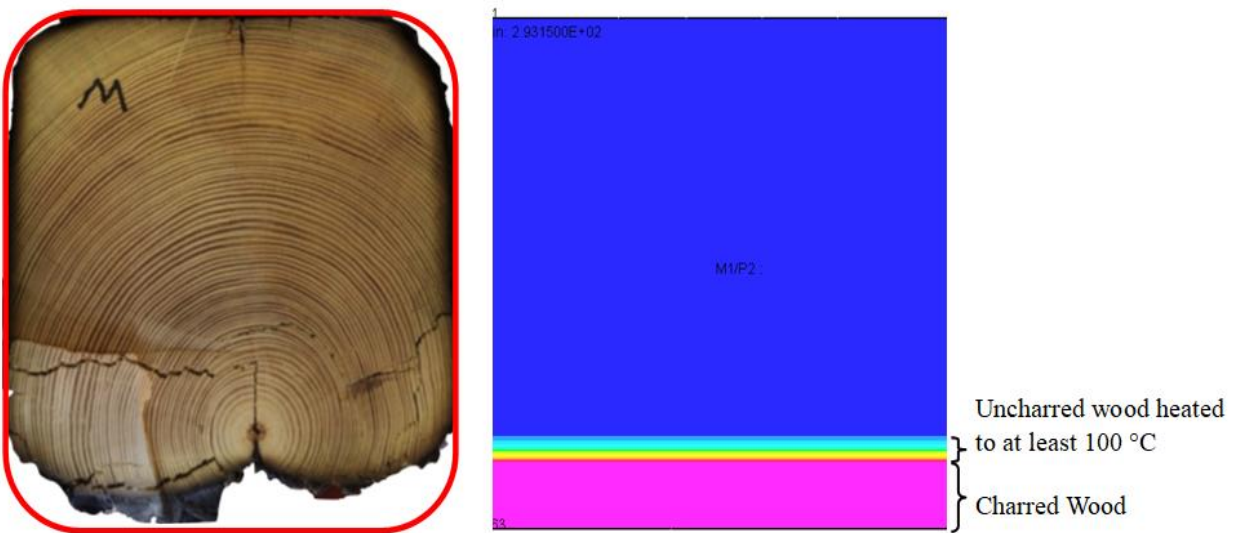
Figure 8.3 Comparison of the charred member and numerical model of a) the Glulam members and b) the heritage members
