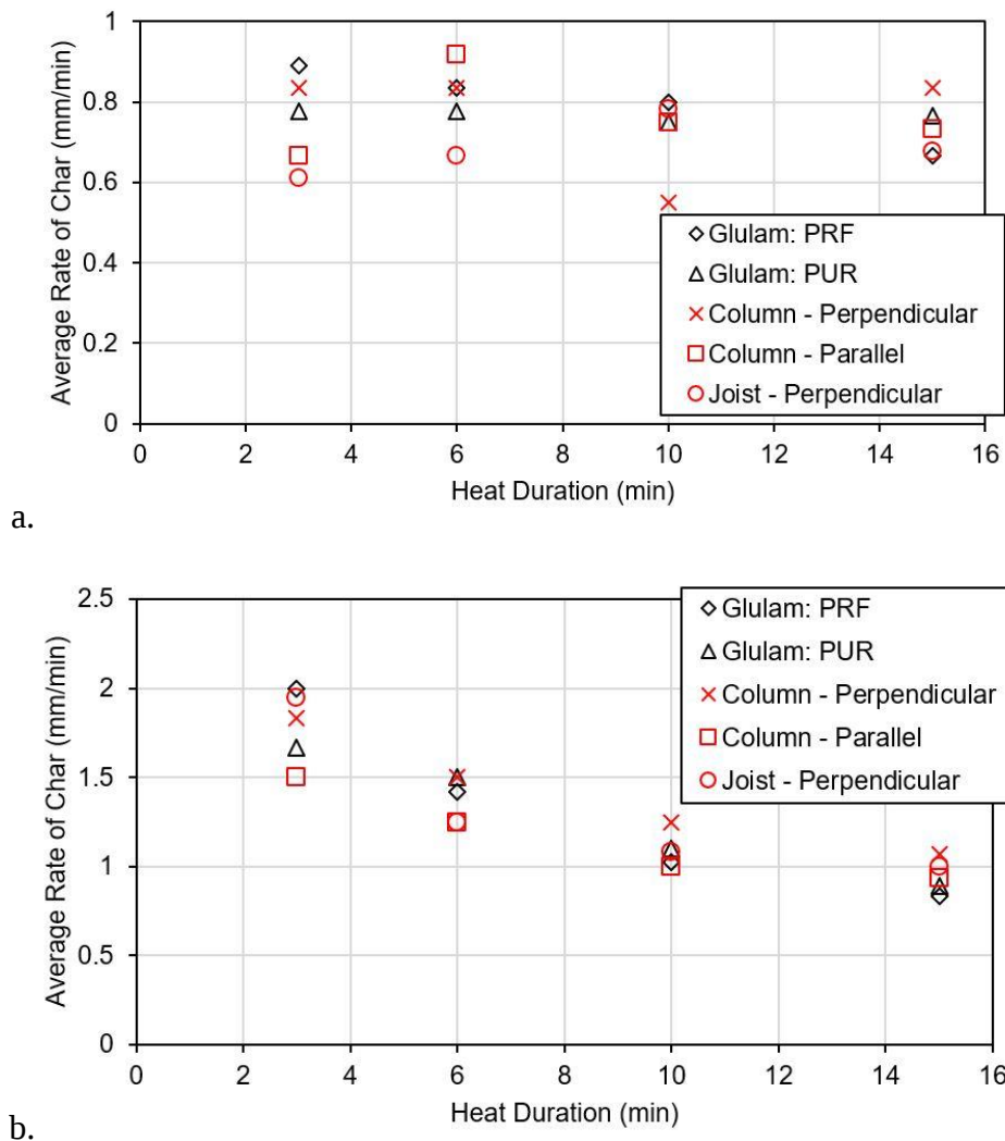
Figure 5.10 The charring rates for the 3, 6, 10 and 15 minute test durations at a. 30 kW/m 2 and b. 50 kW/m 2 .
