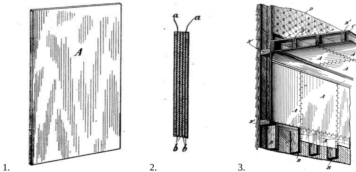
Figure 3.8 Images from Sackett's patent for an interior wall covering, 1. plan view, 2. cross-section view, showing built up layers of paper and calcined gypsum, and 3. possible applications of the boards (from [50]).
