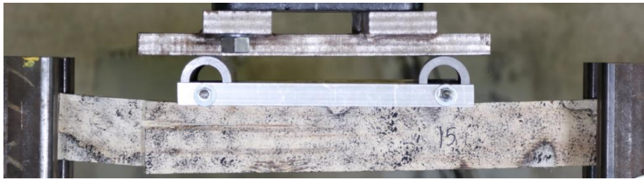
Figure 7.5 Failure of an LVL beam, carved to the 10 mm damage state.
