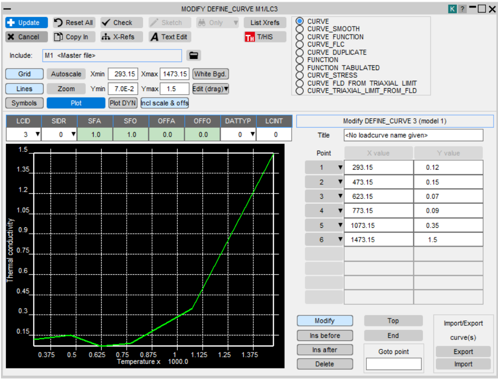
Figure A.3 Defining a curve (thermal conductivity shown here).
