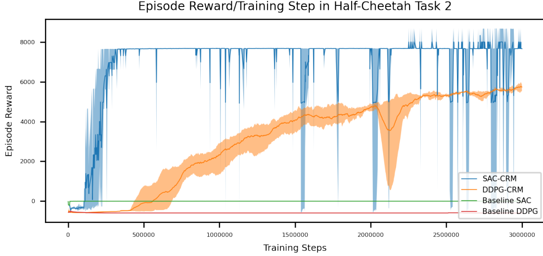
Figure 5.8: CRM vs baselines in Half-Cheetah Task 2
