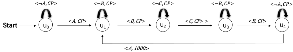
Figure 5.3: The RM automaton of Task 2 in the Half-Cheetah domain.
