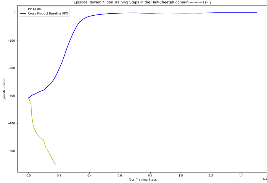
Figure 5.12: PPO-CRM vs baseline PPO in Half-Cheetah Task 2
