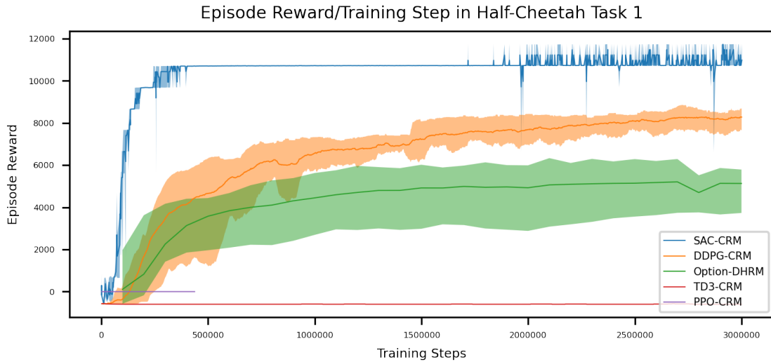
Figure 5.9: Results for Task 1 in the Half-Cheetah domain
