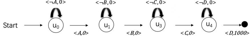
Figure 3.2: The automaton of the RM environment example
