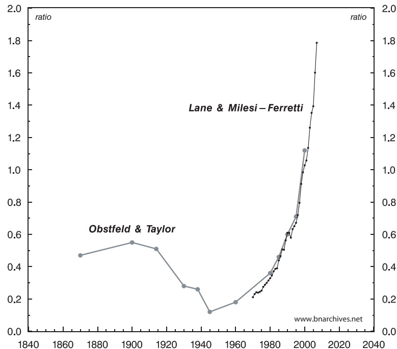
FIGURE 5 Ratio of Global Gross Foreign Assets to Global GDP
