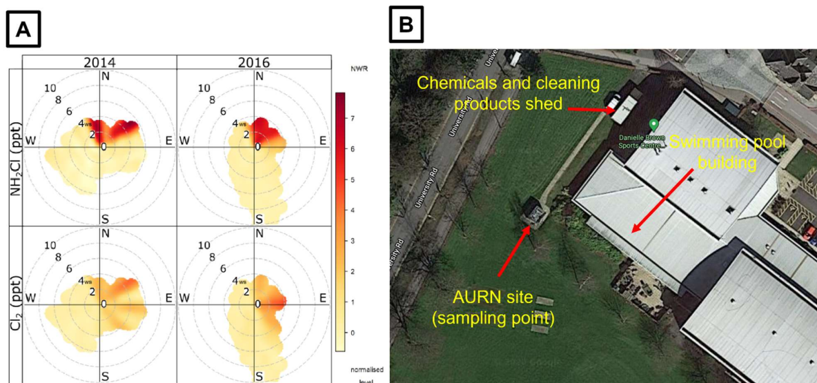
Figure 2: Polar plots of \text{Cl}_2 and \text{NH}_2\text{Cl} for August 2014 and February 2016 (Panel A). An aerial view of the sampling site is also shown (Panel B). Data included in the analysis has been restricted to \text{Cl}_2 and \text{NH}_2\text{Cl} above LOD.
