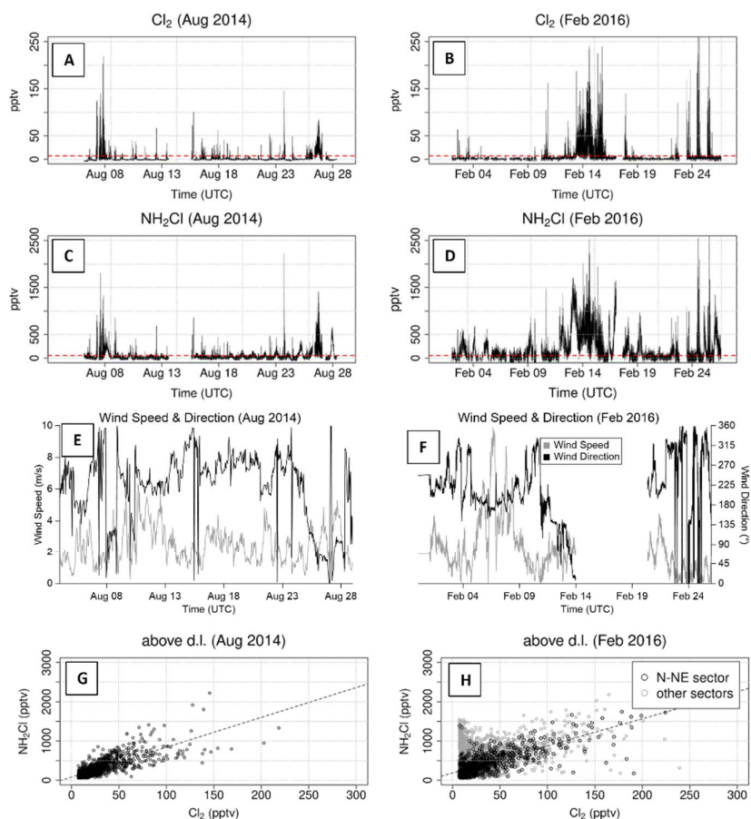
255 Figure 1: Ambient \text{Cl}_2 and \text{NH}_2\text{Cl} data for August 2014 (A, C) and February 2016 (B, D). Wind speed and wind direction are displayed for 2014 (E) and 2016 (F) as well. \text{NH}_2\text{Cl} mixing ratios are also plotted against \text{Cl}_2 mixing ratios for 2014 (G) and 2016 (H) where the observations are filtered for \text{Cl}_2 data above LOD. The horizontal red-dashed lines represent analyte detection limits in the time series. The presented r^2 values in Panel H are for N-NE sector.
