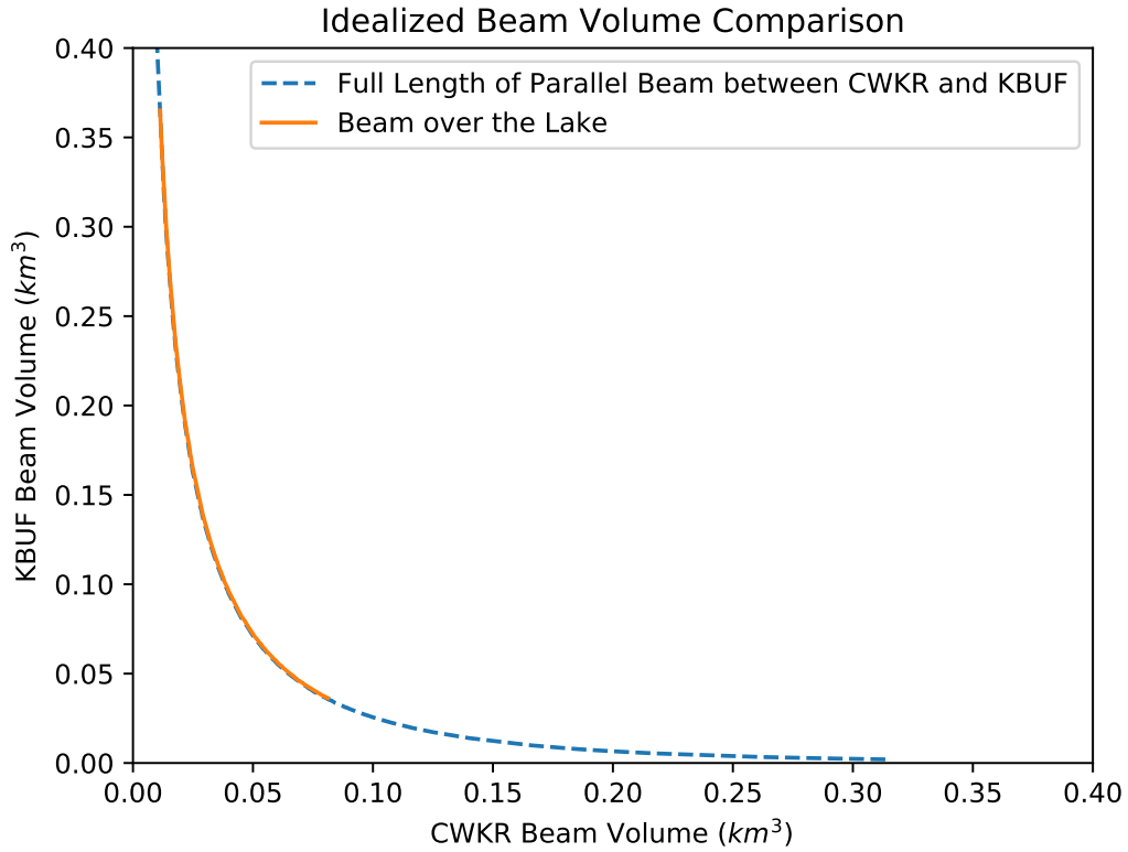
Figure 4.1: Gate-by-gate idealized beam volume comparison along a straight line between radars, assuming Gaussian beam functions.
