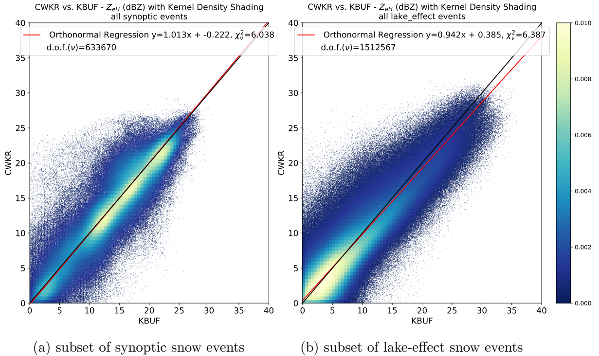
Figure 3.41: Scatter-plots of CWKR versus KBUF grid analyzed reflectivity, with Kernel Density Estimation shading. The red line is an Orthonormal Linear Regression, with a black identity line.
