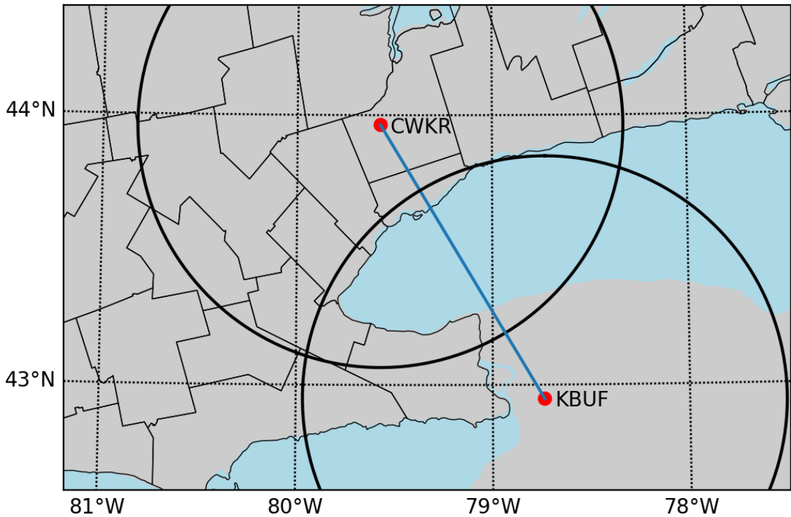
Figure 1.1: The location of the NWS Buffalo Radar (KBUF) and King City Radar (CWKR) are shown as red dots, with a 100 km range ring around each. The distance between the two, drawn as a blue line, is 131.5 km.
