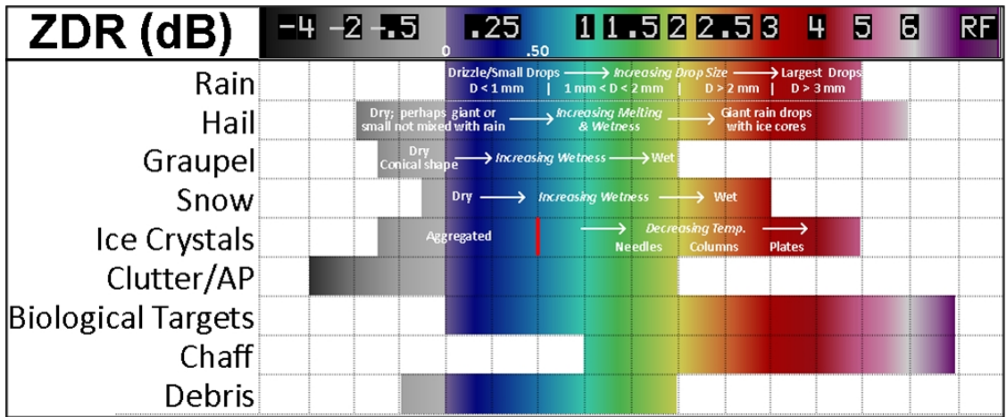
Figure 1.2: Chart of expected ranges of Z_{DR} for a variety of targets. Taken from Fabry (2015).
