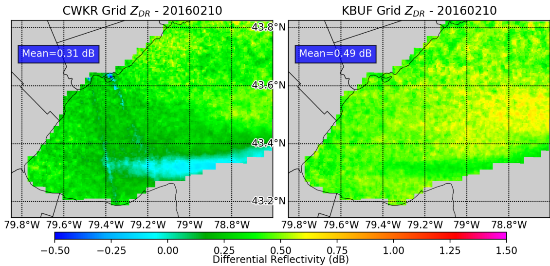
Figure 3.34: Gridded Z_{DR} comparison for 10 February 2016. Time-average of all admitted scans.
