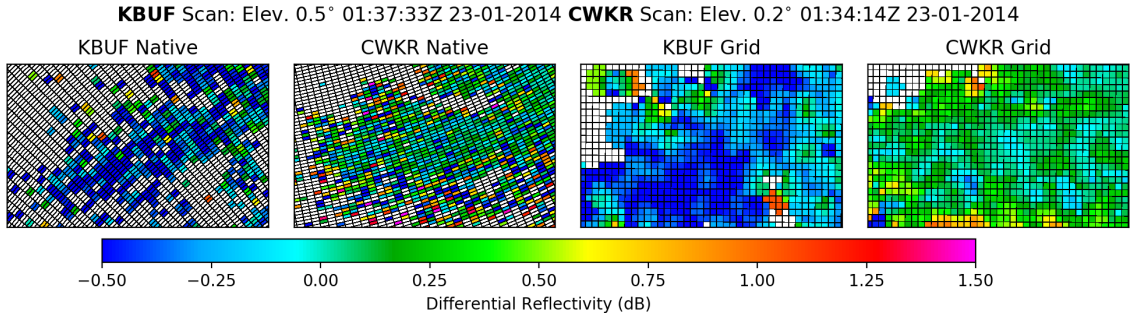
(b) Z_{DR} comparison, in contrast with (a), shows the limitations of representing a non-linear field with an isotropic distance-weighting function.
