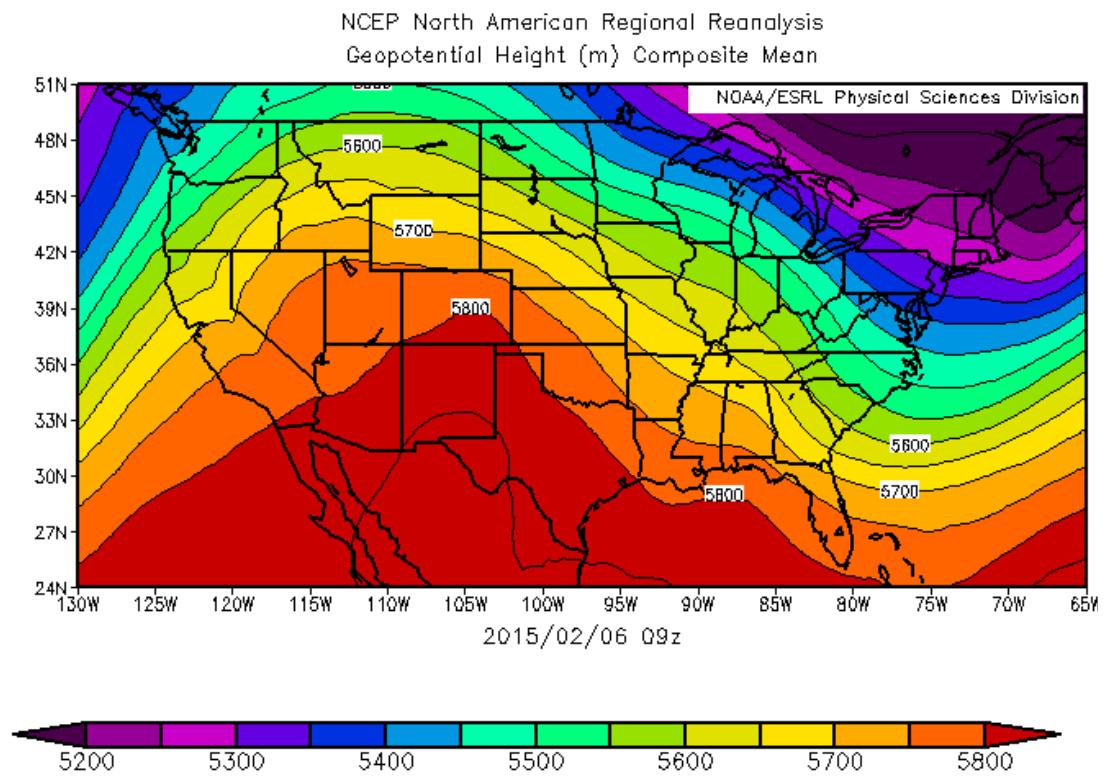
Figure A.6: 500mb Geopotential Height at 09Z 6 February 2015.
