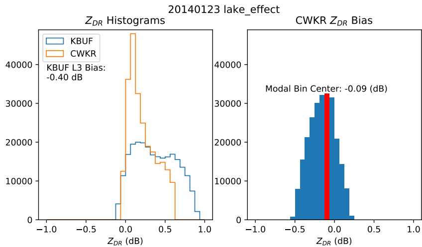
Figure 3.8: Histograms of Z_{DR} (left), Z_{DR} bias at CWKR (right). Bias is calculated by subtracting the gridded, bias-adjusted Z_{DR} at KBUF from the Z_{DR} at CWKR. Both datasets use the 50th percentile as a threshold. The modal bin is shaded red.
