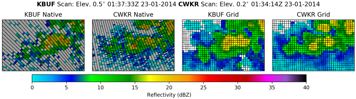
(a) Z_H comparison, shows the transformation from a smooth input to smooth gridded output.
