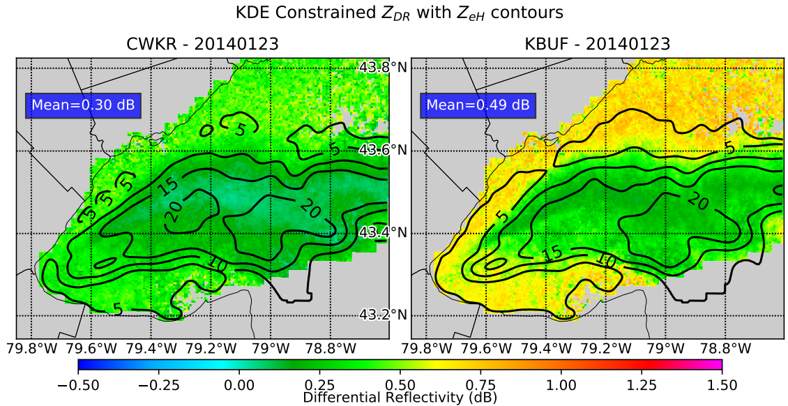
Figure 3.43: Comparison of gridded Z_{DR} with Gaussian ( \sigma = 3 ) smoothed contours of Z_{eH} for 23 January 2014. Z_{DR} is constrained by only including points above the 50th percentile KDE.
