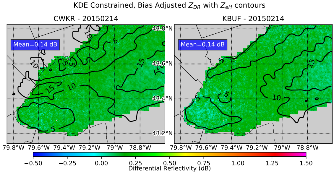
Figure 3.49: Comparison of gridded Z_{DR} with Gaussian ( \sigma = 3 ) smoothed contours of Z_{eH} for 14 February 2015. Z_{DR} is constrained by only including points above the 50th percentile KDE, and is bias-adjusted
