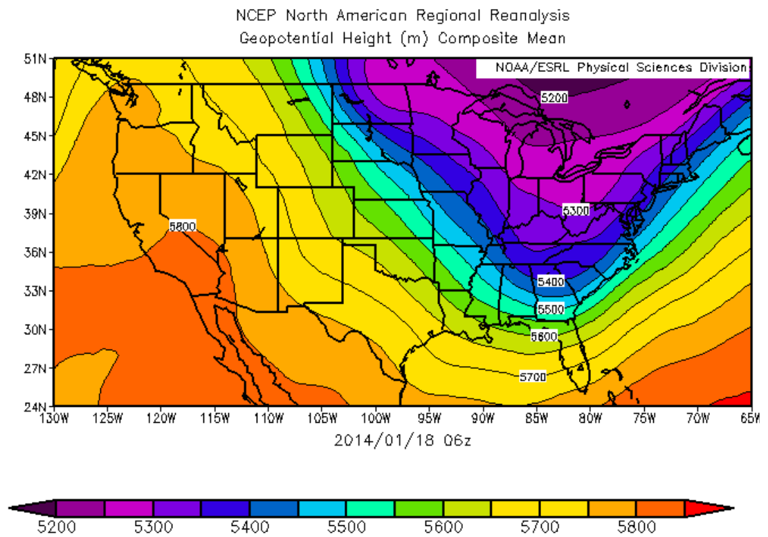
Figure A.1: 500mb Geopotential Height at 06Z 18 January 2014.
