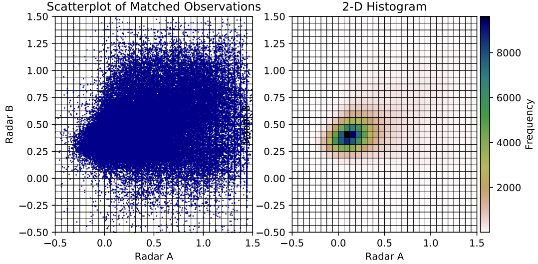
Figure 2.3: Scatter-plot of matched points illustrating the high density of the points (left). The total of points in this figure are 147,457. 2-D histogram of the same matched points, binned to native data resolution (right).
