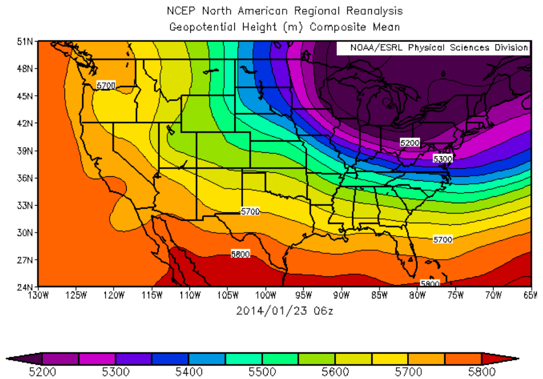
Figure A.2: 500mb Geopotential Height at 06Z 23 January 2014
