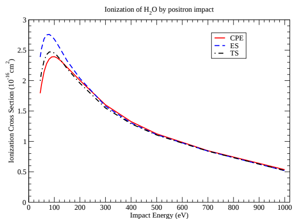
Figure 2. Cross-sections for the direct ionization of the \text{H}_2\text{O} molecule by positron impact, calculated in the framework of the CPE, ES and TS models. At the date of the study there were no experimental data for the direct ionization of this target.
