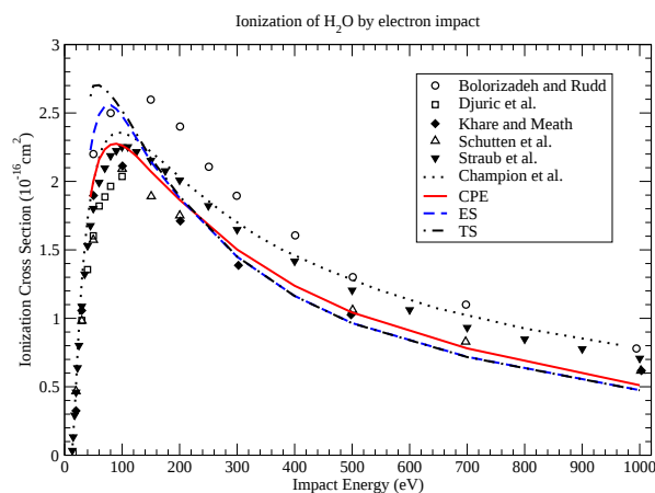
Figure 1. Cross-sections for the direct ionization of the \text{H}_2\text{O} molecule by electron impact, calculated in the framework of the CPE, ES and TS models, compared with the measurements of [8, 9, 10, 11] and the theoretical results [19] and [20].
