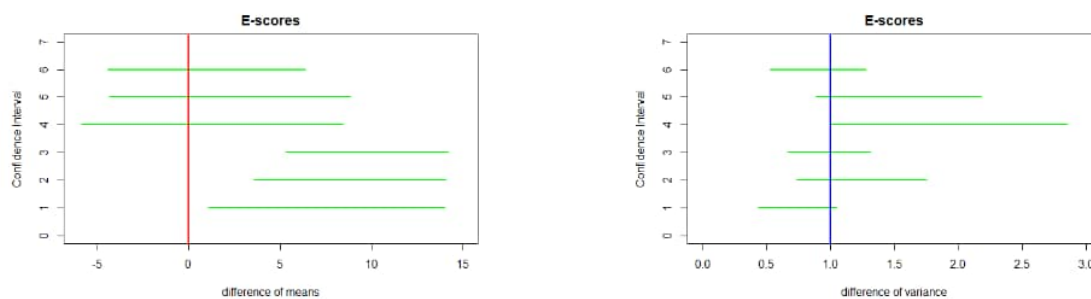
Figure 4: Comparing means and variances
