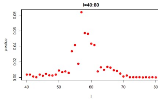
Figure 3: Variation of p-values
