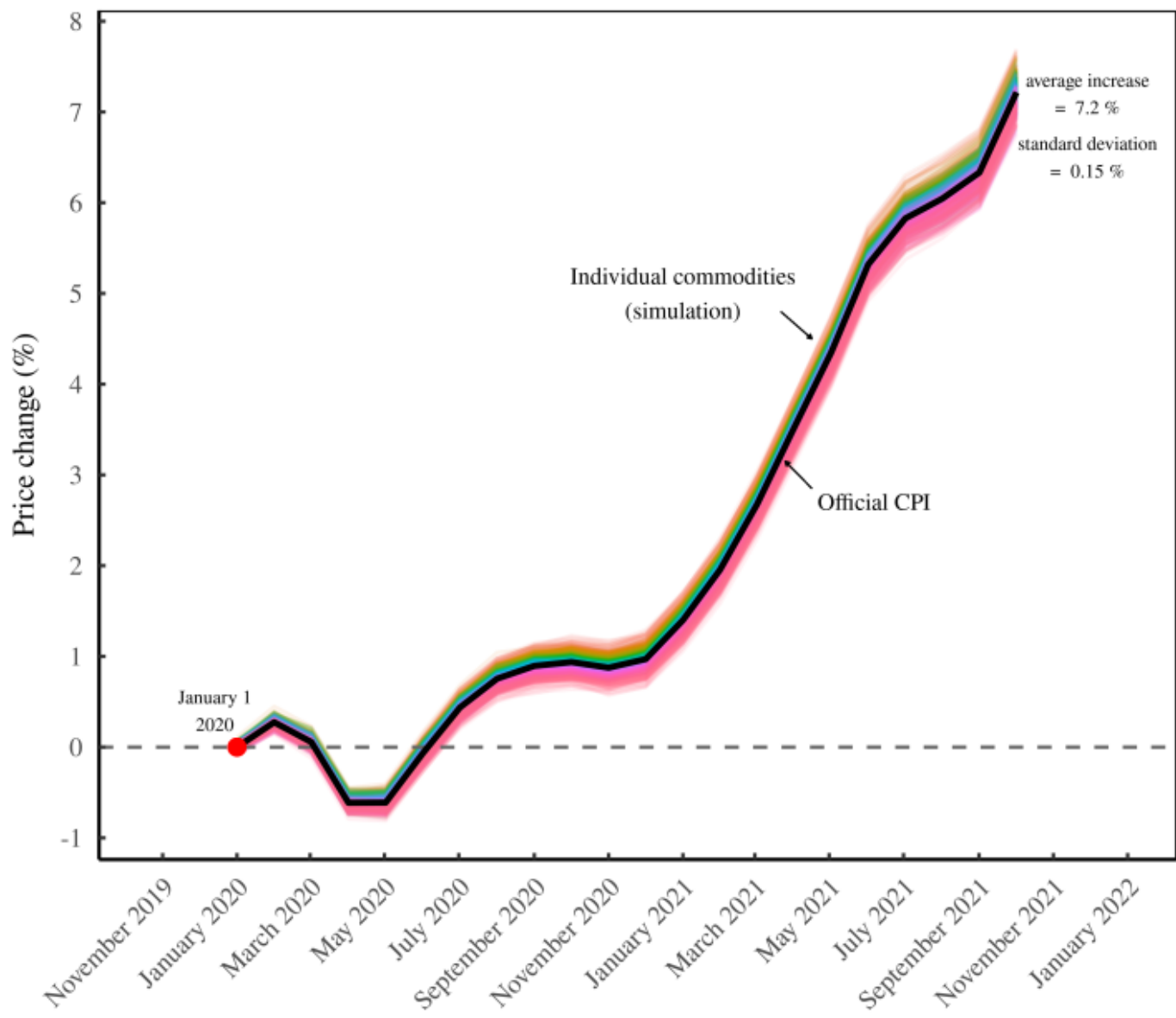
Figure 2: What price change would look like if inflation was nearly uniform across commodities. The black line shows the change in the actual US consumer price index. The colored lines show what the price-change of individual commodities would look like if inflation was nearly uniform.
