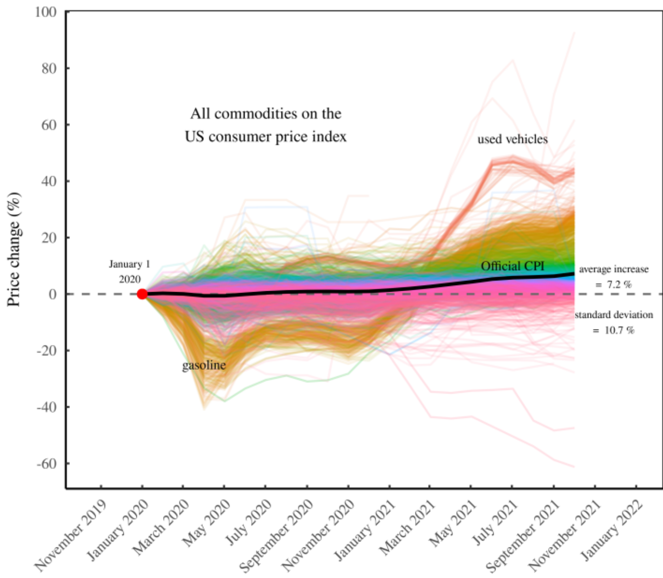
Figure 3: Price change in the real world. The black line shows the change in the US consumer price index since January 1, 2020. The colored lines show the indexed price of all the individual commodities tracked by the CPI. Many commodities are tracked in multiple locations. [ Sources and methods ]
