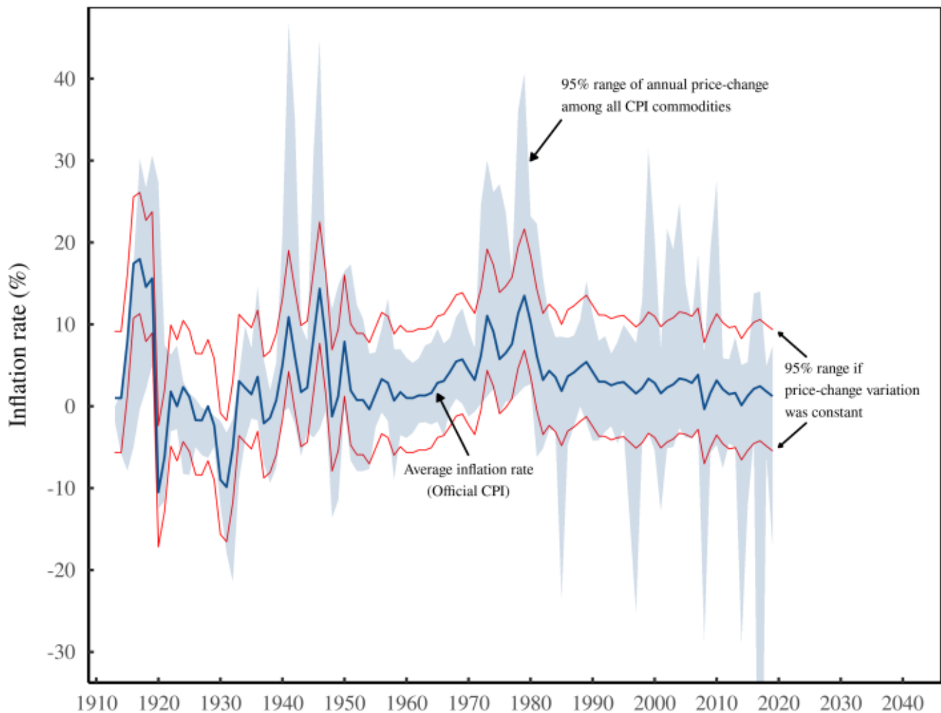
Figure 7: Is price-change variation constant over time? The blue lines and the shaded region reproduce (from Figure 6) the real-world trends in US prices. The red lines show what price-change variation would look like if it was constant over time at the US historical average. [ Sources and methods ]
